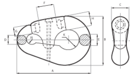
PEAR SHAPED END SHACKLE
